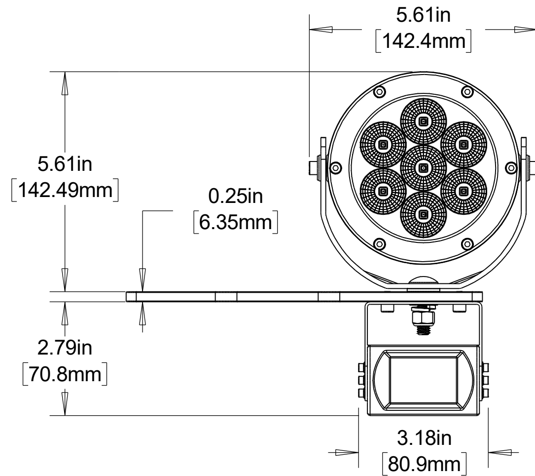
EXM LIGHT & VIDEO KIT DIMENSIONAL DRAWING (FOR REFERENCE ONLY)
