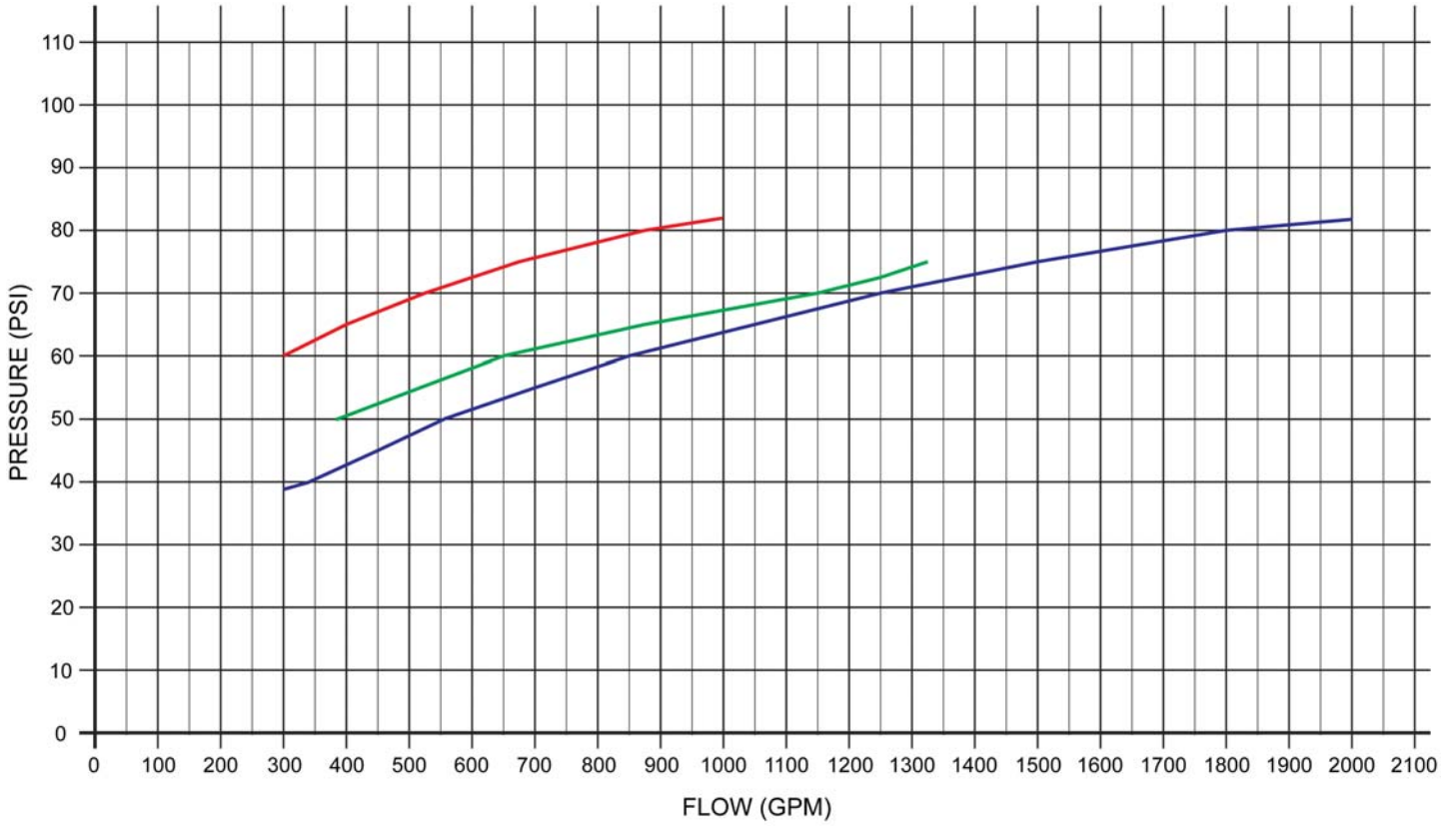
DISCHARGE DATA
