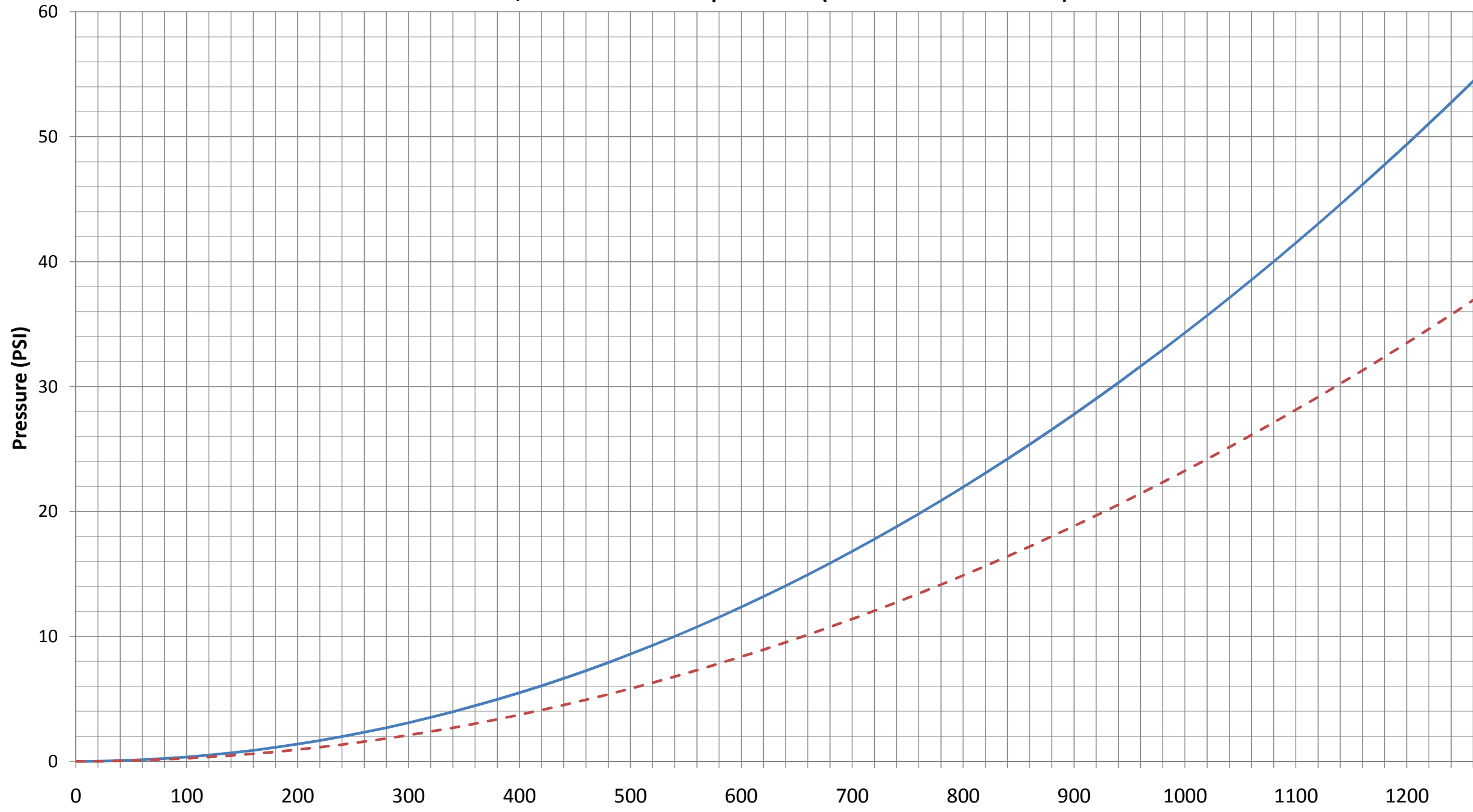
283-A, 283-B Stream Shaper Losses (3.5" inlet & 2.5" outlet )
