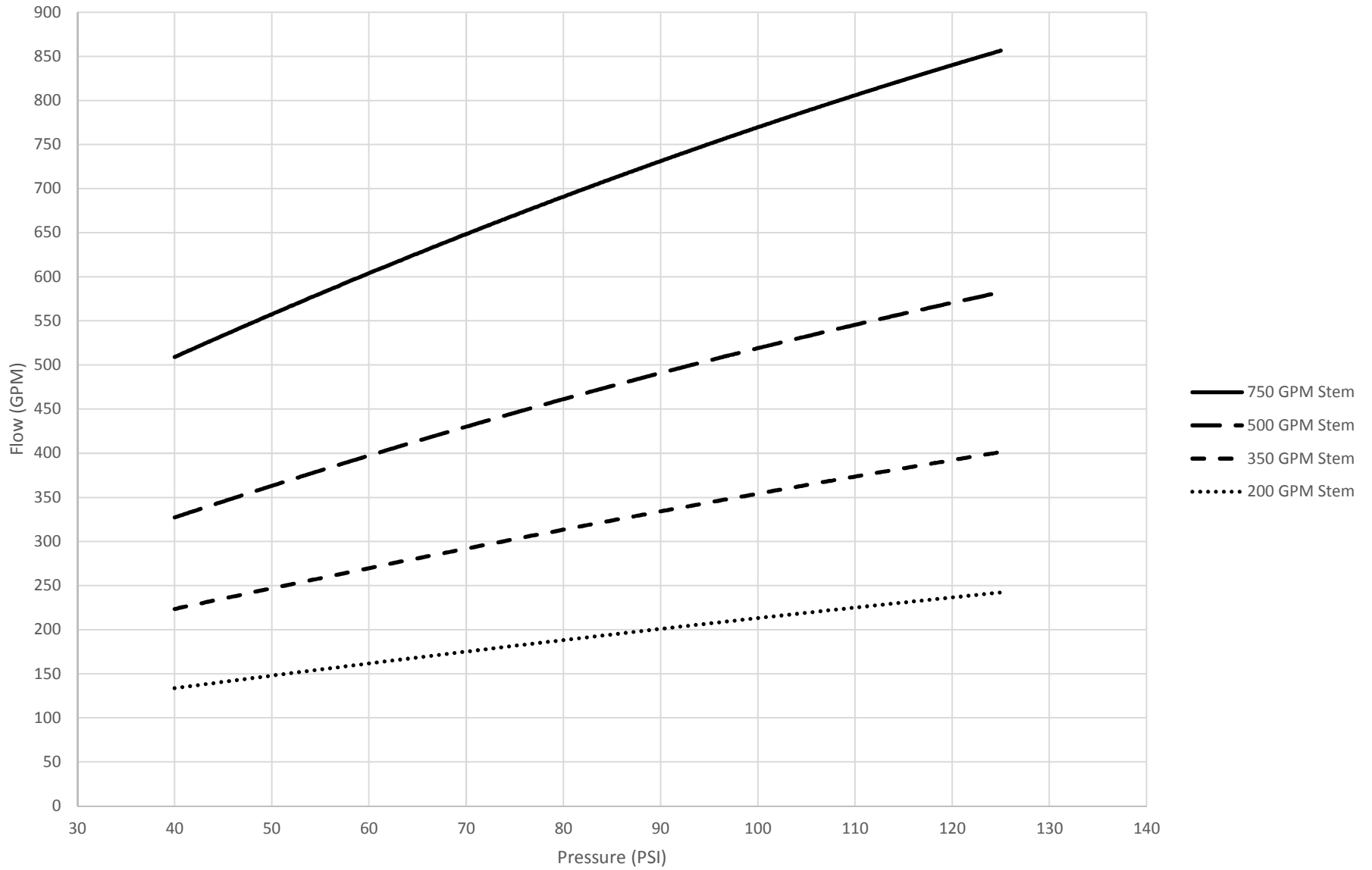
7000-EHD Nozzle Pressure vs. Flow
